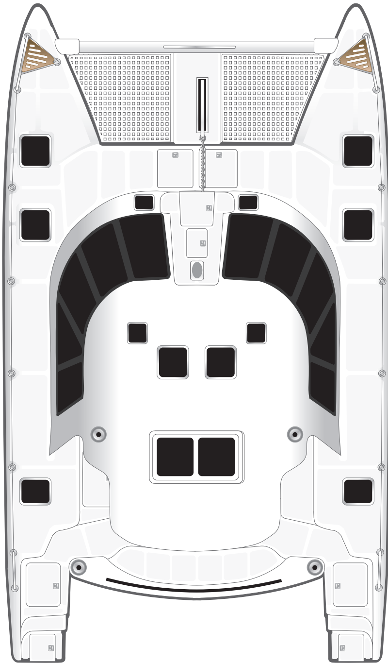
Layout Option 1: Central steering station & downstairs galley. Forward bathroom and laundry.
