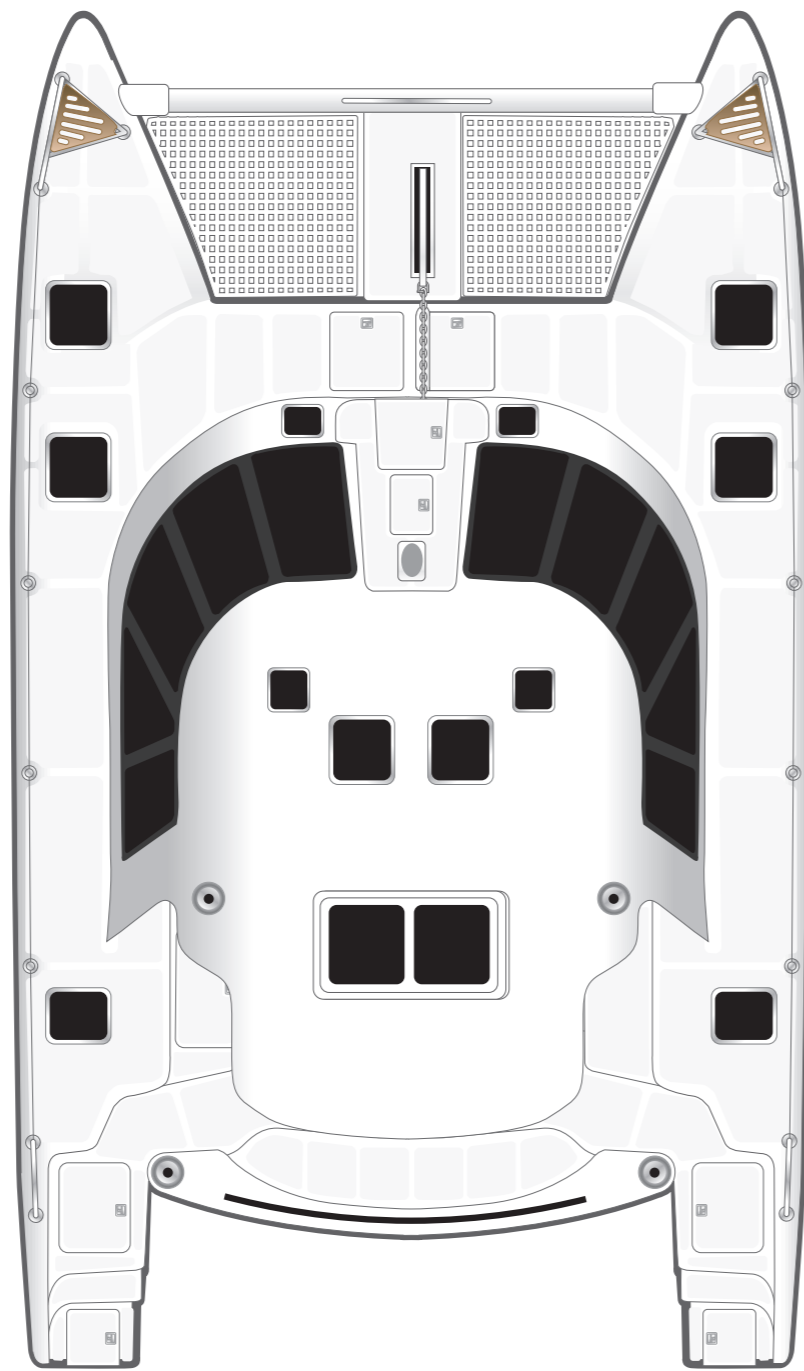
Layout Option 2: Offset steering station, upstairs galley & forward walk through wardrobes.
